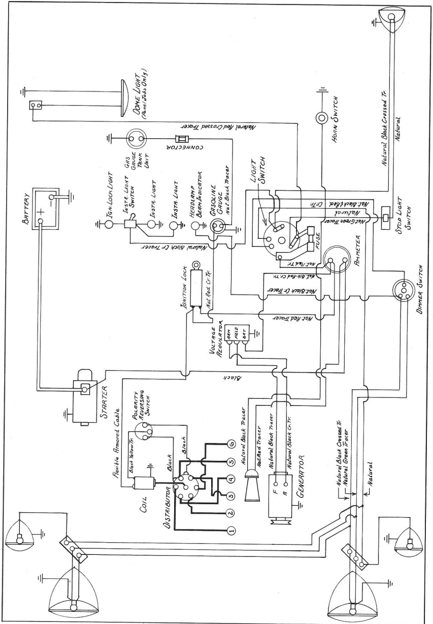
Fig. 47—Simplified Wiring Diagram
